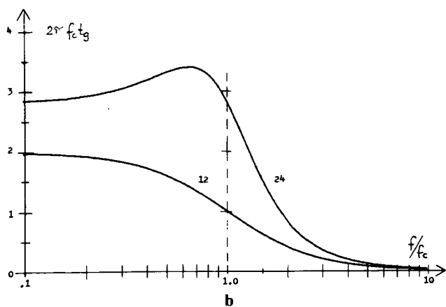
Fig. 6. Optimum crossover function response. a. Amplitude response. b. Group delay response.
