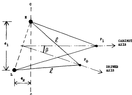
Fig. 1. Radiation from two sources H and L which are separated by a distance d_1 and offset by d_2 in their planes of radiation.
