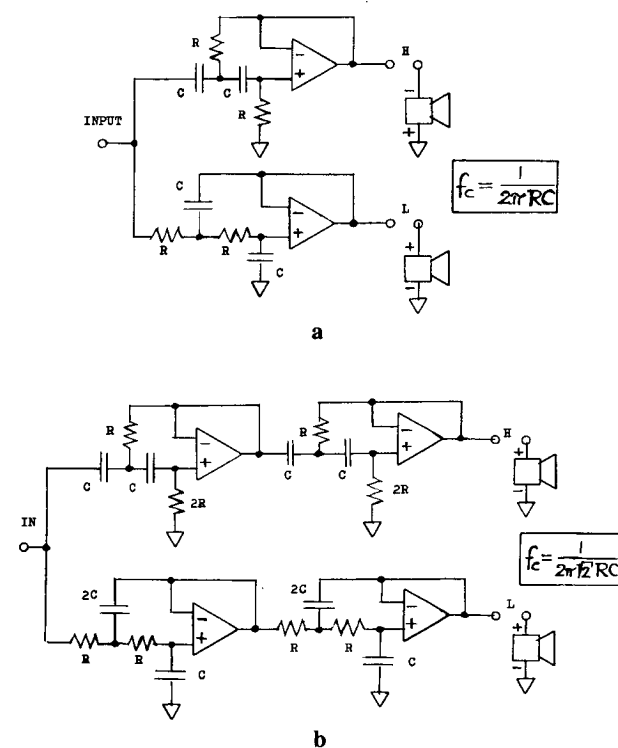
Fig. 5. Realization of optimum crossover function. a. 12-dB per octave filter. b. 24-dB per octave filter.
