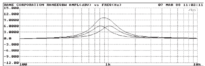
Figure 9. Summed response of adjacent filters showing combining or interpolation between bands for proportional-Q equalizer.
