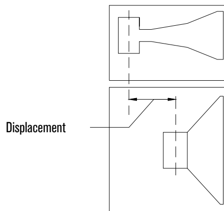
Figure 3. Vertical Driver Displacement
