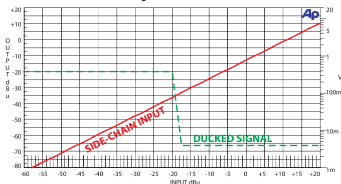
Figure 5: Ducker
