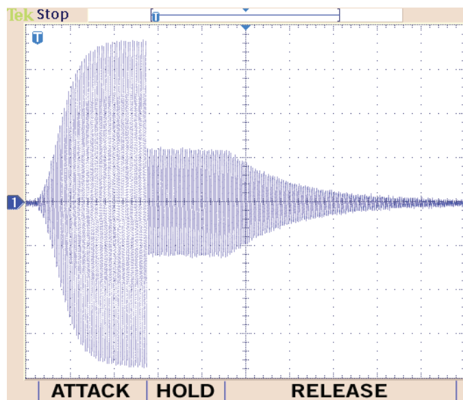
Figure 1: Gate Envelope
